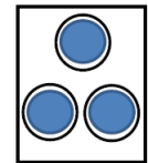
Rated current 800A 300 MCM x 3 37 strands each
