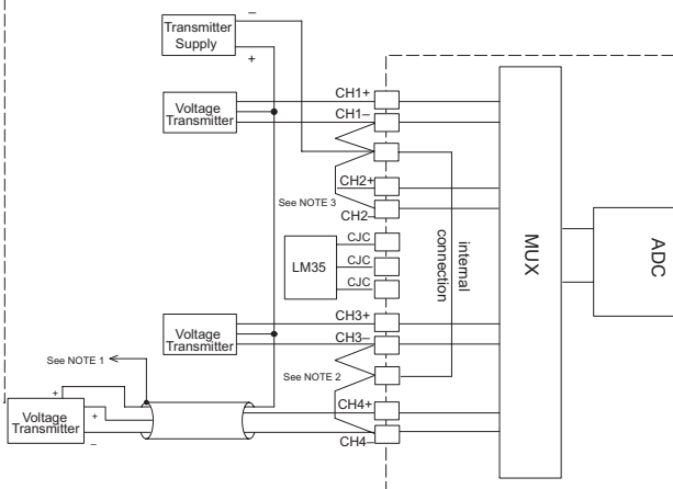
Voltage Input wiring diagram
