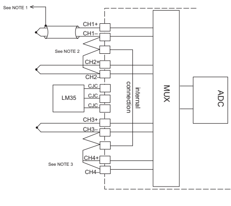
Thermocouple Input wiring diagram
