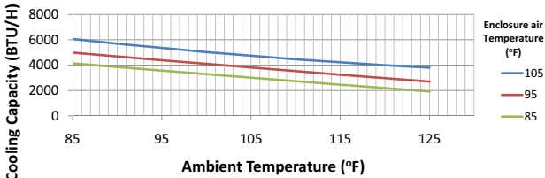
TA10-060-16-xx
