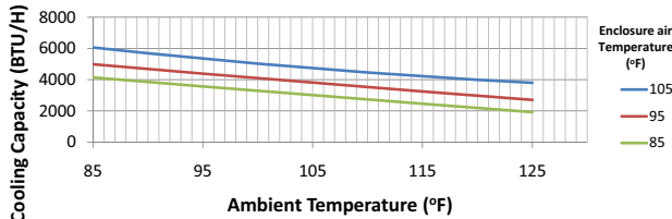
TA10-060-26-xx TA10-060-46-xx
