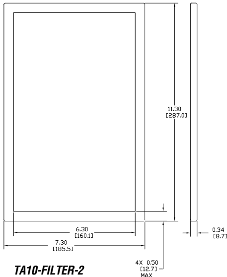
TA10-FILTER-2
