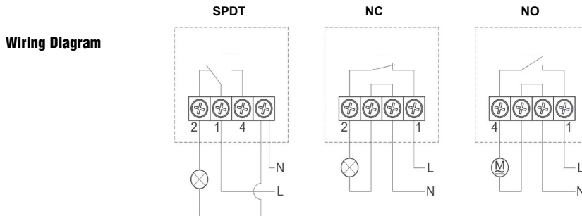
Wiring Diagram
