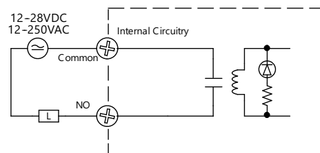
Typical Circuit
