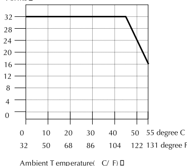
Derating Chart
