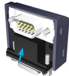
DL06 15-pin high density D-sub port adapter DO-06ADPTR
