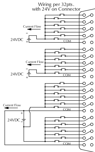
Connector Pins
