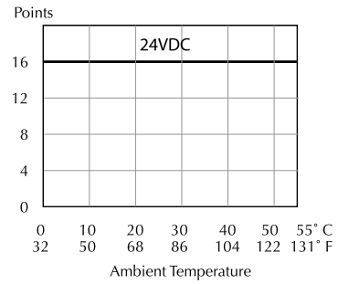
Derating chart
