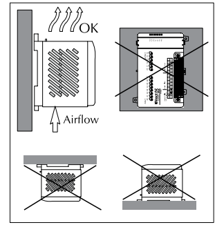
Mounting orientation
