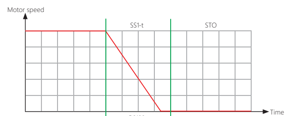
Figure 1.2: SS1-t behavior
