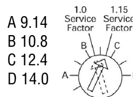
Example of 12.0 FLA setting for heater pack number H2011B showing position for 1.0 or 1.15 service factor motors.
