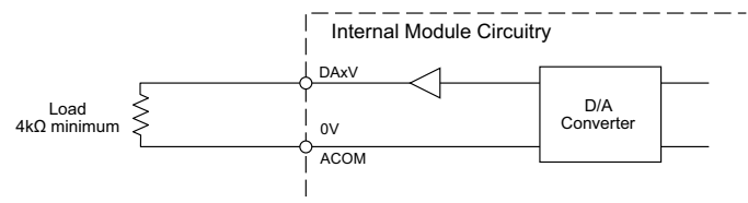
Analog Voltage Output Circuit
