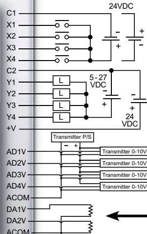
Wiring Diagram
