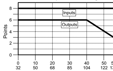
C0-01AR-D Temperature Derating Chart
