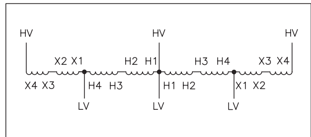
Wiring Diagram 10
