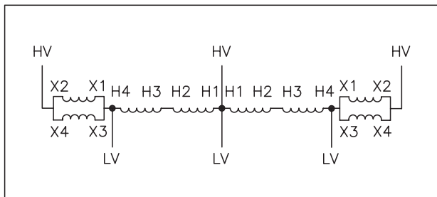
Wiring Diagram 9
