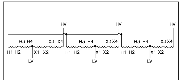
Wiring Diagram 8
