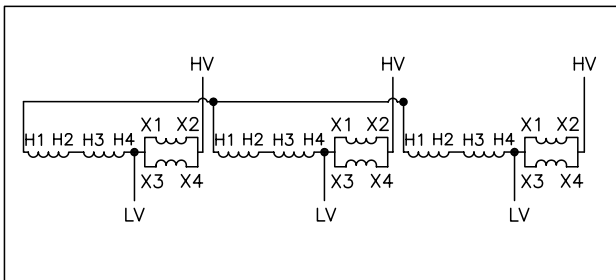
Wiring Diagram 7
