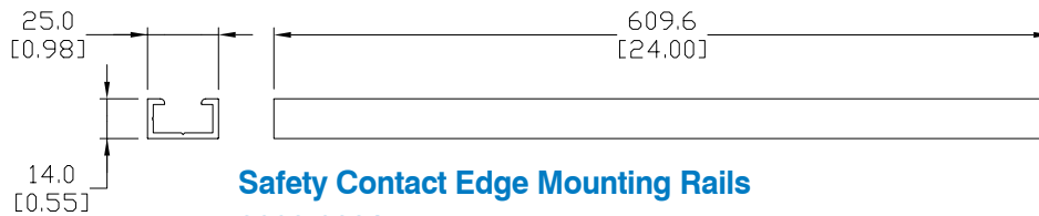
Safety Contact Edge Mounting Rails 2002-0230
