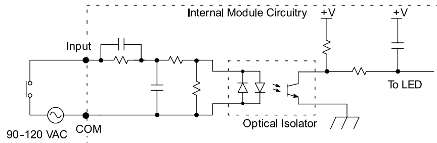
Equivalent Input Circuit
