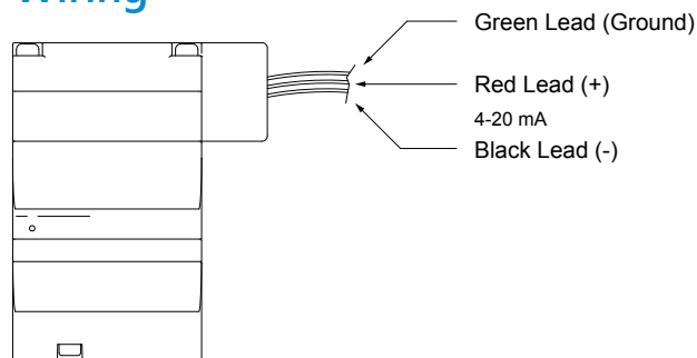
NCP2-20-xxxN units with wire leads
