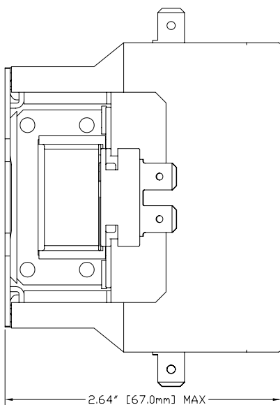
Side Detail
