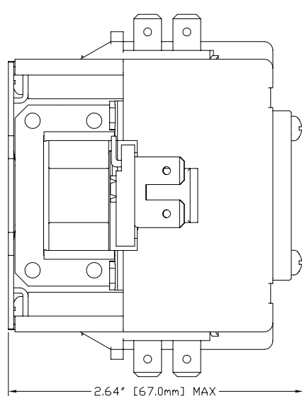
Side Detail
