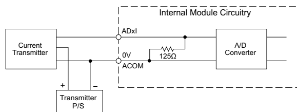
Analog Current Input Circuit
