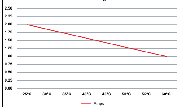
BX-xxTA Derating Chart
