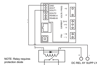
RELAY OUTPUT
