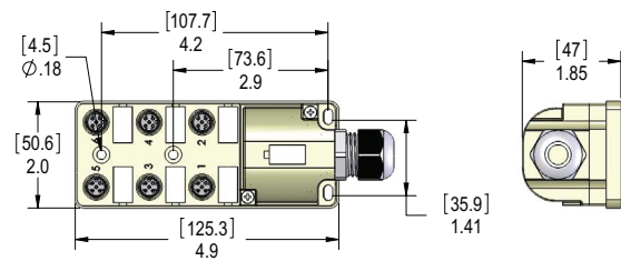
Figure 3: 6-Port, 4-Wire/5-Pole
