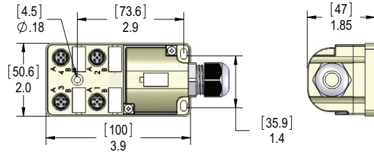
Figure 2: 4-Port, 5-Wire/5-Pole
