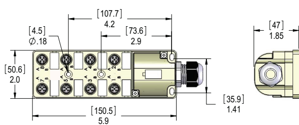
Figure 6: 8-Port, 5-Wire/5-Pole
