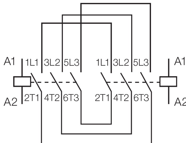
Reversing Bar Connection Kit Electrical Wiring Diagram
