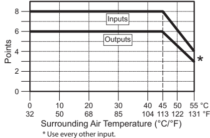
C0-10DRE-D Temperature Derating Chart
