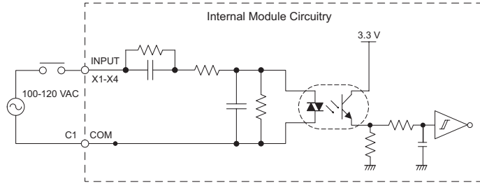
Equivalent Discrete Input Circuit
