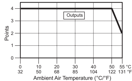
C0-12DRE-1-D Temperature Derating Chart
