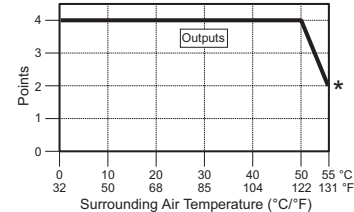
C0-02DR-D Temperature Derating Chart
