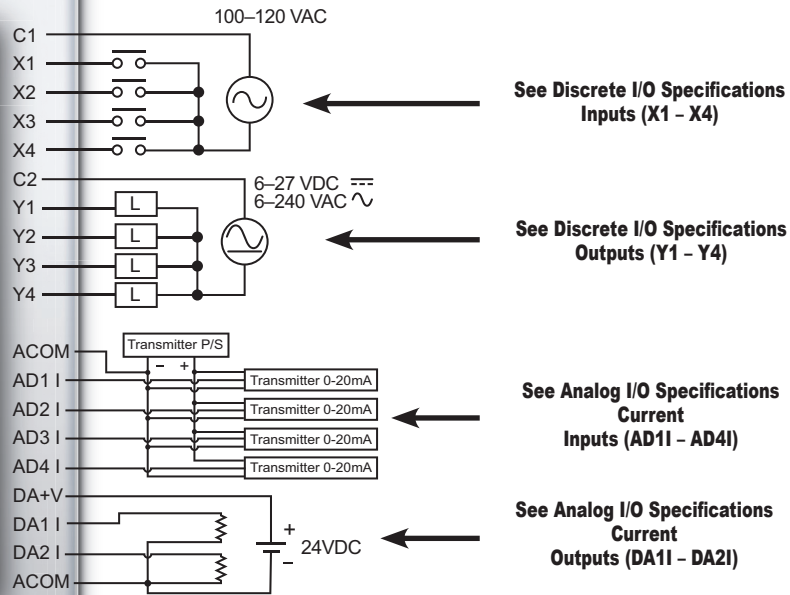
Wiring Diagram
