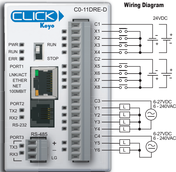
Wiring Diagram
