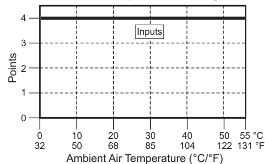
C2-08D2-4VC Temperature Derating Chart
