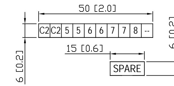
ZL-RTB20 CUT-OUT LABEL DIMENSIONS
