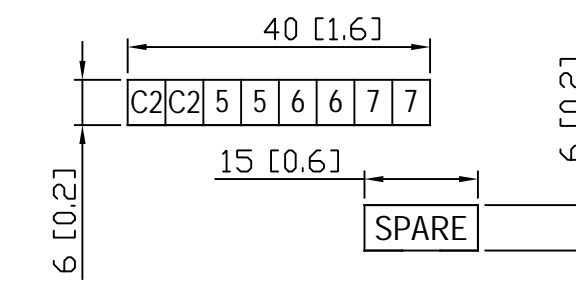
ZL-RTB20-1 CUT-OUT LABEL DIMENSIONS
