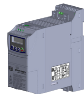
Figure A2: (c) Retract the lower snaps of the filter set into the CFW300 base (c) Retraer as trabas inferiores del conjunto filtro en la base del CFW300 (c) Recolha as travas inferiores do conjunto filtro na base do CFW300
