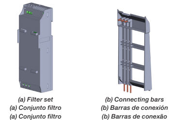
Figure A1: (a) and (b) Parts of the CFW300-KFA filter kit
