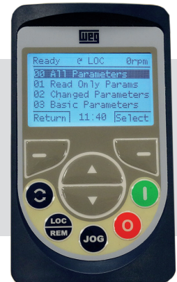
HMI-01 Advanced Text Remote Keypad
