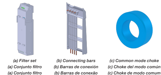
Figure A1: (a) to (c) Parts of the CFW300-KFB-T4 filter kit
