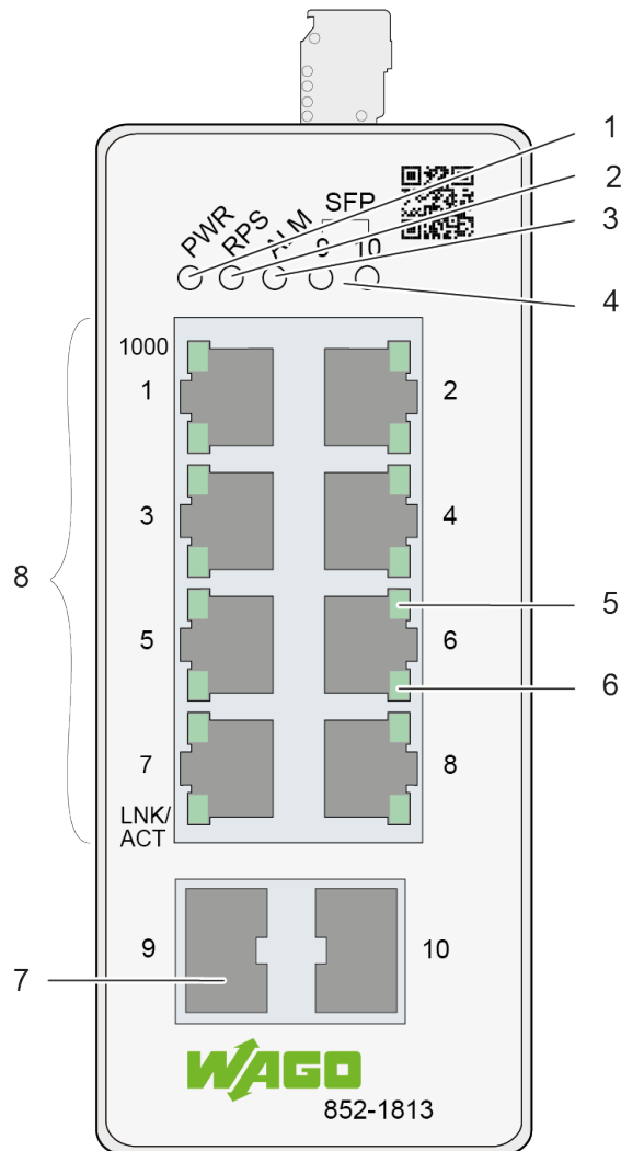
Figure 1: Front View of the Lean Managed Switch
