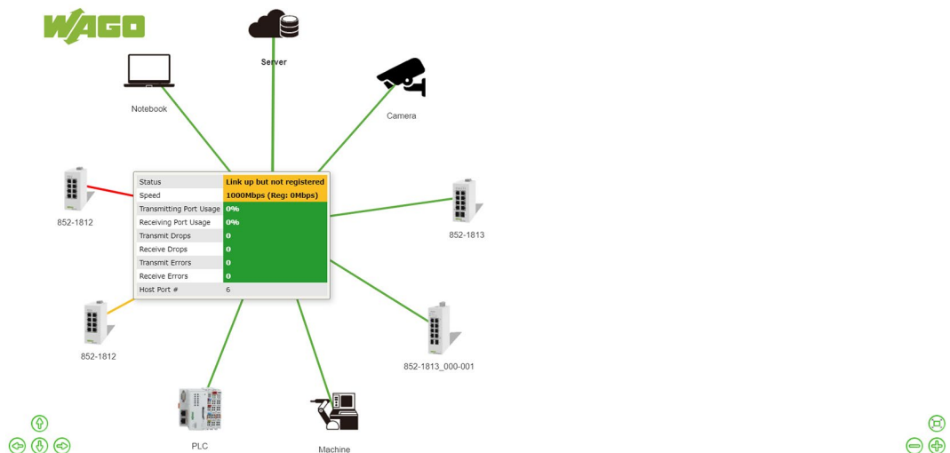
Figure 32: Topology Map – Link not registered
