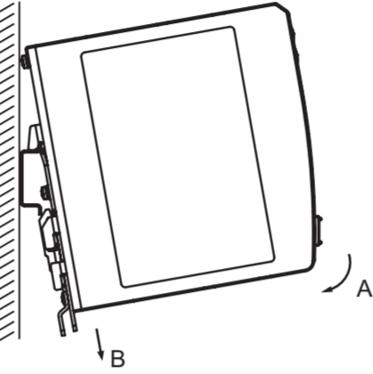
Figure 1 : montage
