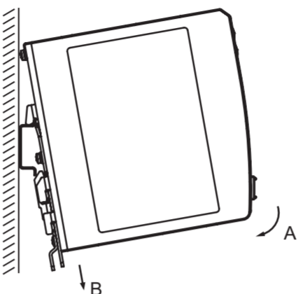
Figure 1: Mounting
