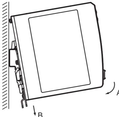
Figure 1: Mounting
