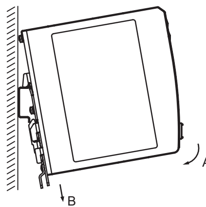
Figure 1: Mounting
