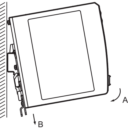
Figure 1 : montage
