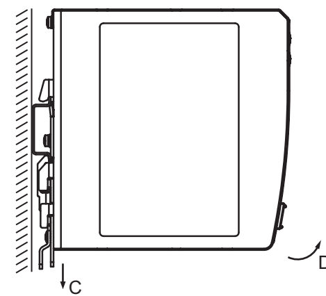
Figure 2: Removal
