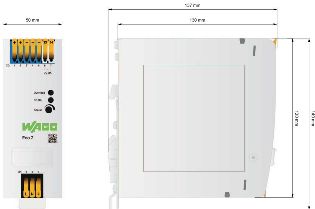
Figure 7: Dimensions
