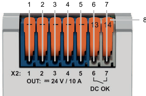
Figure 4: Terminations – Output Side
