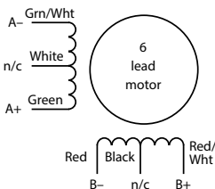
6 Leads Series Connected
