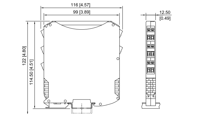
Spring clamp terminal
