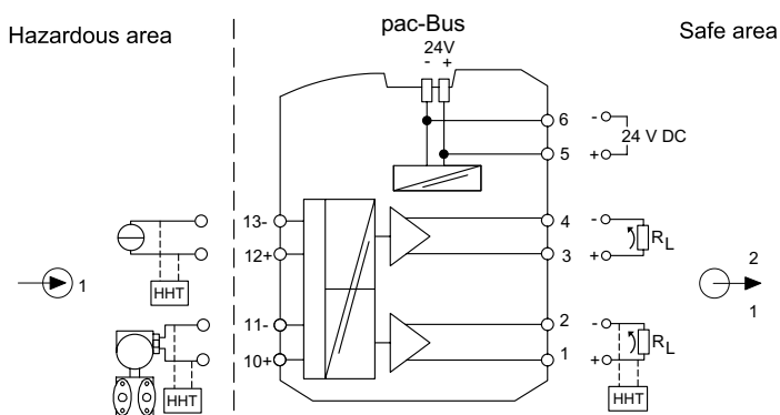
Connection diagram 9260/19-11-10
