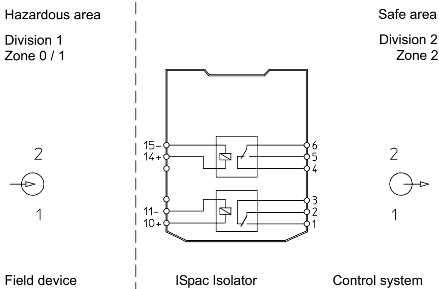
Connection diagram 9172/20-11-00
