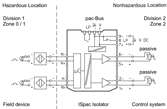
Connection diagram 9146/20-11-11
