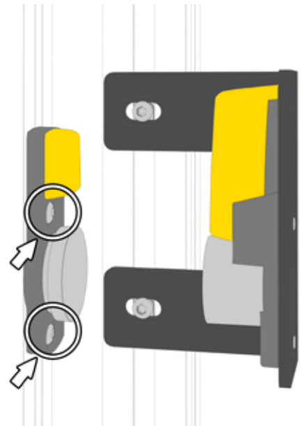
Fig. 9: Attach the anchor plate to the profile of the sliding door and align it with the magnetic guard lock. Tighten the Torx screws M6 x 10 mm.
