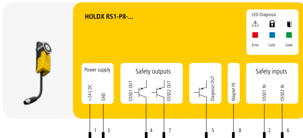
Fig.1: Coded, electronic magnetic guard lock with safety sensor, which is actuated contactlessly by a coded anchor plate. The safety sensor monitors the position of rotating, laterally movable or removable protective devices with the coded electronic anchor plate.
