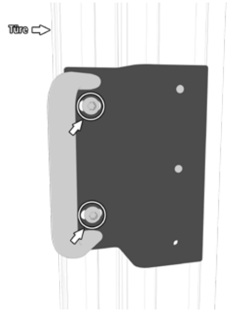
Fig. 6: Attach the mounting plate with the anchor plate to the profile and align with the magnetic guard lock. Tighten the Torx screws M8 x 12 mm.
