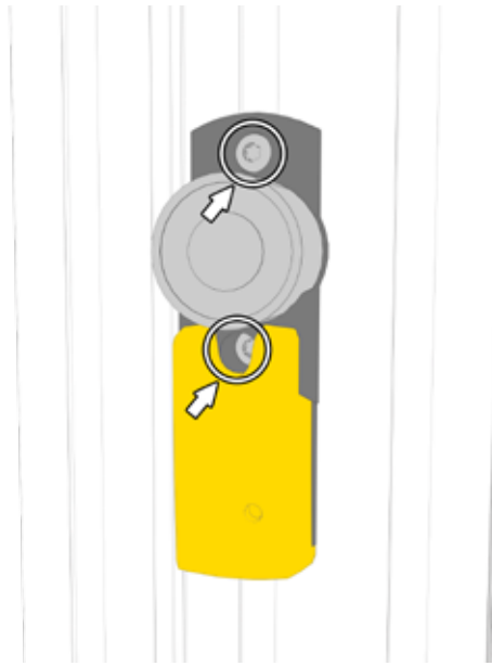
Fig. 4: Attach the magnetic guard lock to the profile at the desired height and tighten the Torx screws M6 x 25 mm.
