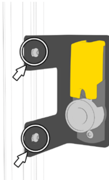
Fig. 8: Attach the mounting plate with the magnetic guard lock to the profile and tighten the Torx screws M8 x 12 mm.
