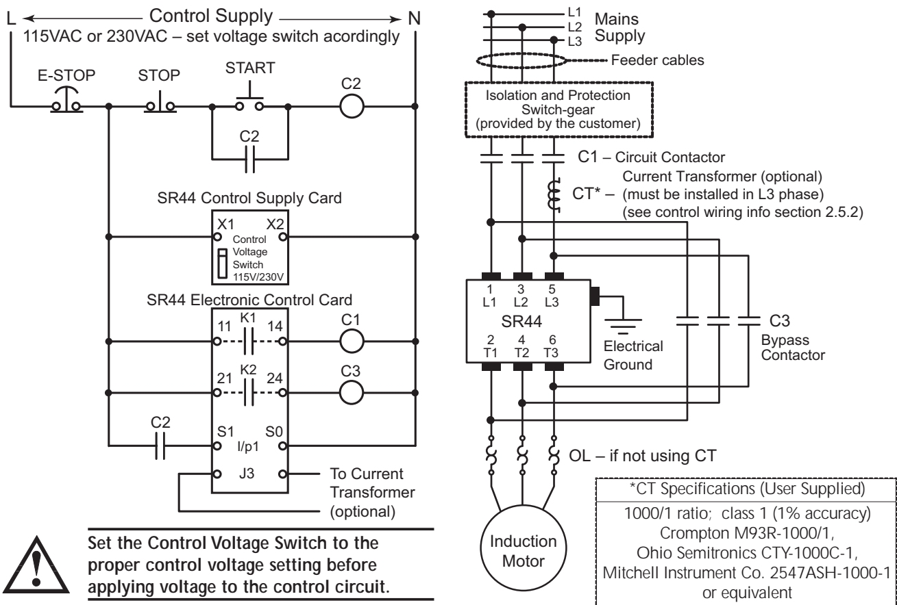
Figure 2.4.1: Power and Contactor Control Circuits for Motor Bypassing
