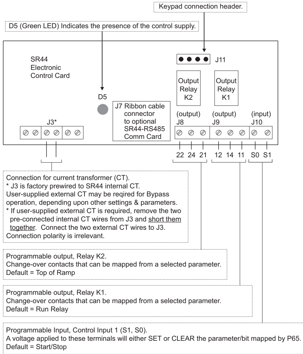
Figure 2.5.2: Electronic Control Card Electrical Connections
