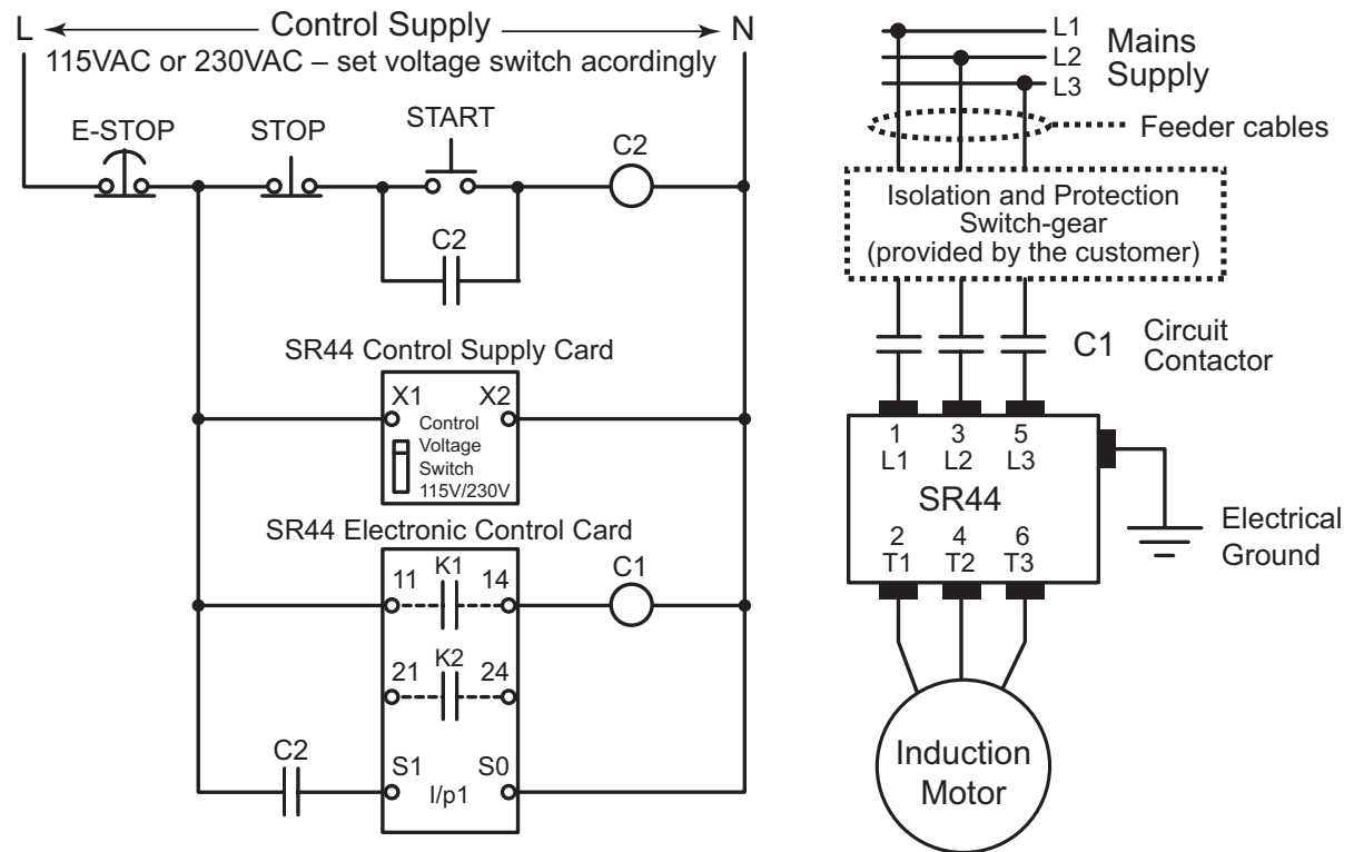
Figure 2.3.1: Wiring Diagram for In-Line Connection of Motors
