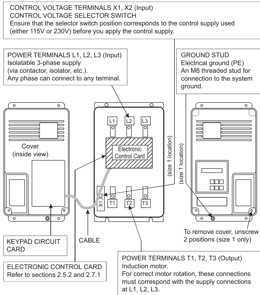
Figure 2.5.1a: SR44 Chassis Size 1 Electrical Connections
