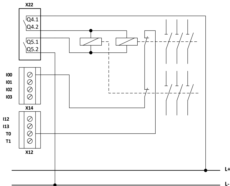
Dual-channel switching relay output with external monitoring – collective feedback
