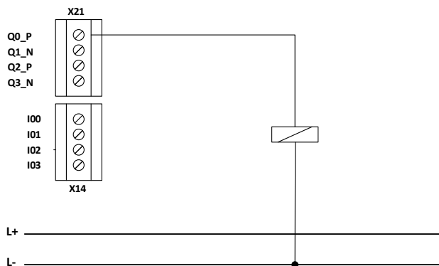
Single-channel switching P output.
