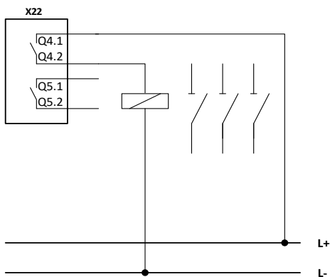
Single-channel switching relay output.
