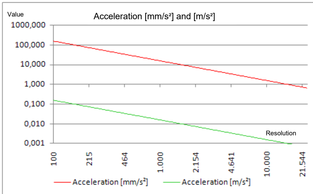
Graph of acceleration resolution, linear (values in mm/s² and m/s²)
