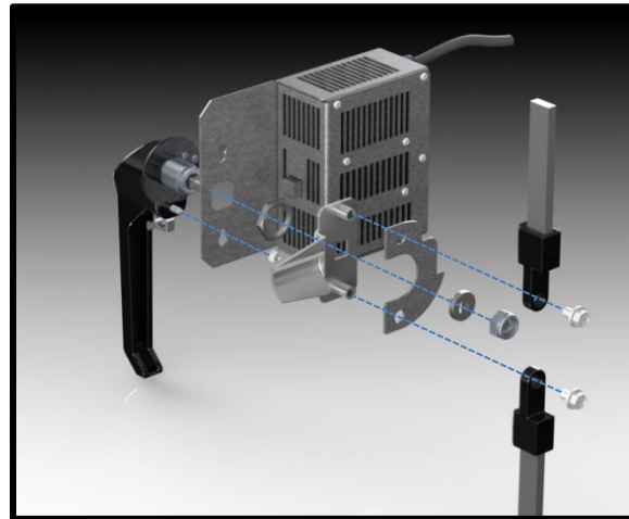
PARTIAL EXPLODED ISOMETRIC VIEW SHOWN 7" SCE HANDLE AND ROD KIT
