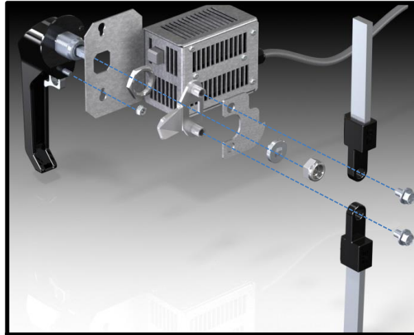
PARTIAL EXPLODED ISOMETRIC VIEW SHOWN 5" SCE HANDLE AND ROD KIT
