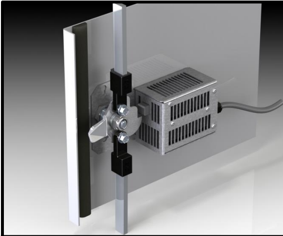
PARTIAL ISOMETRIC VIEW INTERIOR OF DOOR
