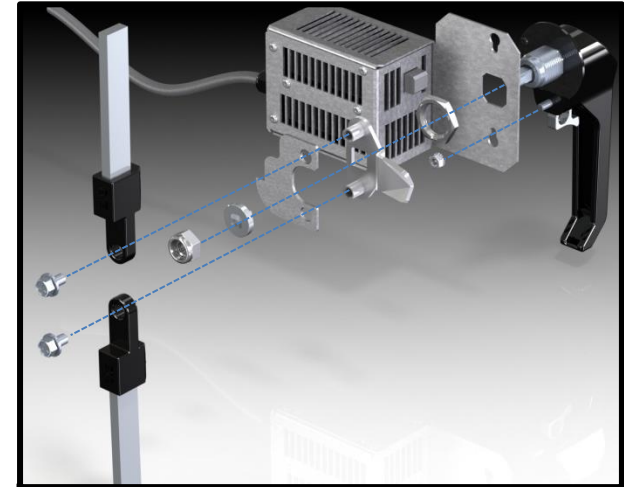
PARTIAL EXPLODED ISOMETRIC VIEW SHOWN RIGHT HINGED
