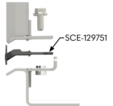
12 Gauge Enclosures 30° Flange Trough Collar
