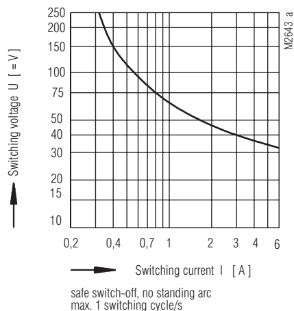
Limit curve for arc-free operation
