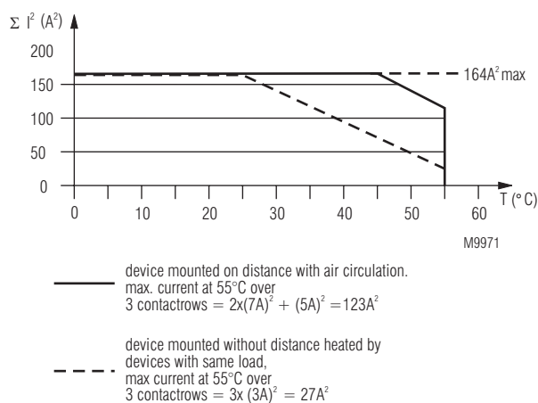
Limit curve for arc-free operation
