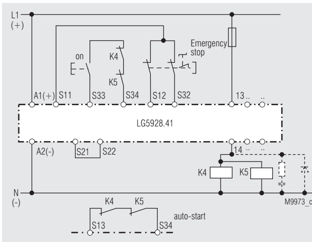
Contact reinforcement by external contactors controlled by one contact path. S33 - S34 must stay open on auto start. Suited up to SIL3, Performance Level e, Cat. 4, if the external contactors are in the same cabinet and the wiring is short circuit and crossfault prove.
